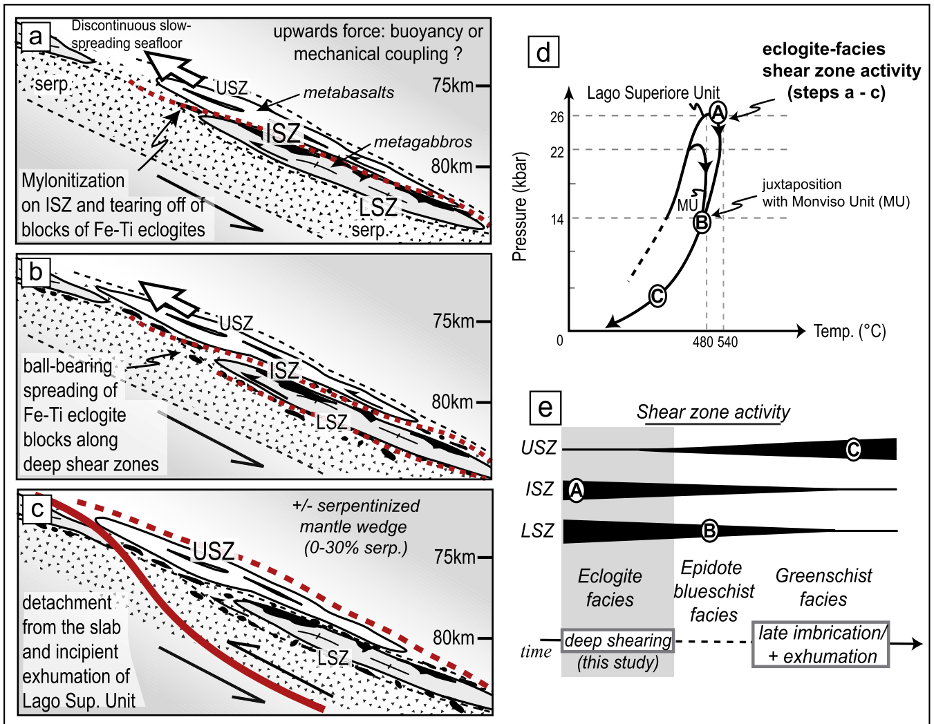
Fig. 10. a. Sketch representing the Lago Superiore ophiolite slice at the onset of mylonitization. Deformation is first localized on the ISZ, at the boundary between basalts and gabbros (red dotted line). b. Ongoing shearing along the plate interface is responsible for dismembering and fragmentation of eclogite blocks detached from the ISZ. c. The whole Lago Superiore unit finally detaches from the downgoing slab and the bulk of the deformation is now localized at the base of the serpentinite sole. Monviso unit, which detaches from the slab at c. 65–70 km is not represented here. d. P–T paths from Angiboust et al. (in press) for both Monviso and Lago Superiore Units. e. Eclogite facies shear zone activity is restricted to the vicinity of peak conditions (i.e. 550 °C, 26 kbar). Juxtaposition with the adjacent Monviso Unit occurs in the epidote blueschist facies during exhumation in the subduction channel (Schwartz et al., 2000). The relative timing of shear zone activity is based on the intensity of metamorphism recorded by the rocks from the different shear zones. (For interpretation of the references to color in this figure legend, the reader is referred to the web version of this article.)
