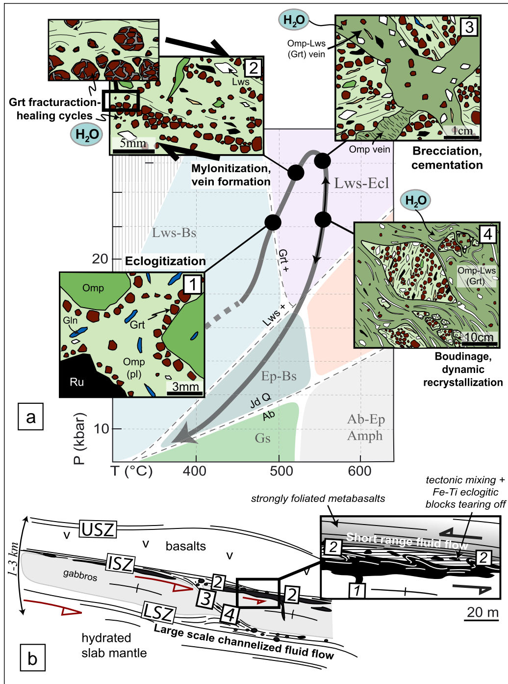
Fig. 8. a. Relative chronology of events (and associated P–T position) observed on eclogite Fe–Ti metabasalt mylonites boudins along the ISZ and LSZ. Igneous texture (step 1) is progressively blurred by mylonitization processes (step 2) leading to grain size reduction, garnet fracturing and phase segregation. Variable amounts of hydrous phases crystallized depending on the amount of water available during mylonitization. Eclogite facies breccias (step 3), commonly found along the LSZ are generally cemented by omphacite +/- lawsonite +/- garnet. These brecciated fragments (Fig. 3f) may be embedded as boudins in a later lawsonite eclogite-facies foliation (step 4). The P–T diagram at the background shows the P–T path for the LSU ophiolite, the location of the main metamorphic facies and the relative position of the four steps identified. Note that the presence of lawsonite (now pseudomorphed by epidote), omphacite and garnet in all textural positions constrains these events to the lawsonite-eclogite facies. b. Schematic drawing at the scale of the Lago Supérieure unit, showing the location of the different shear zones and the location of the four steps mentioned above. Our results indicate that substantial fluid flow occurred along the LSZ, whereas only short range localized fluid flow within the ISZ.
